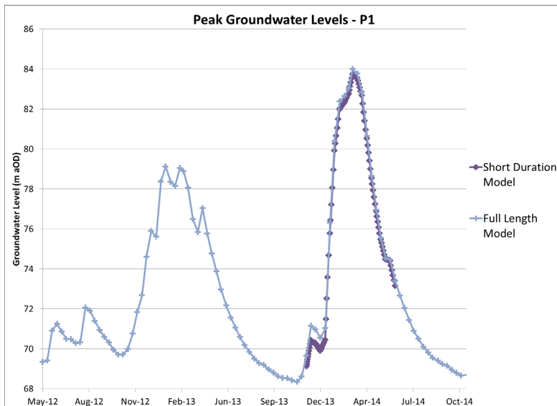
Figure 2 P1 Peak Groundwater Levels
