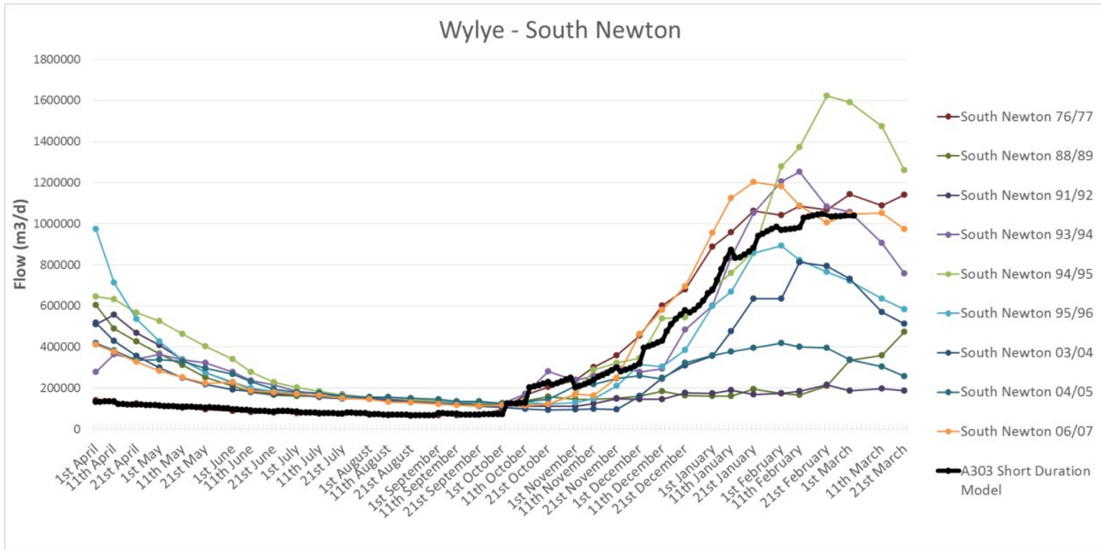
Figure 5 River Wylfe at South Newton - Series of Dry and Average Years
