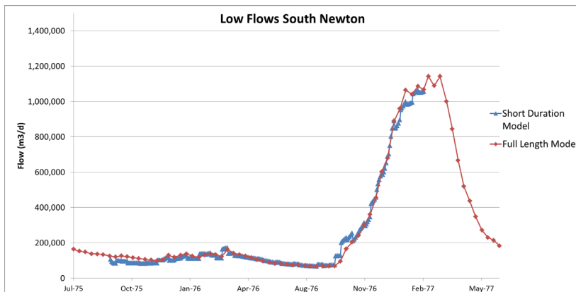
Figure 4 Wylfe at South Newton Low Flows
