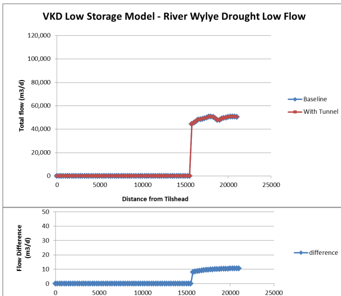
Figure 21 Accretion Plot for Low Flows in River Wylye in low storage model
