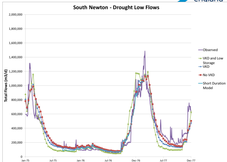
Figure 12 Comparison of River Wylfe Flows at South Newton with different model parameters
