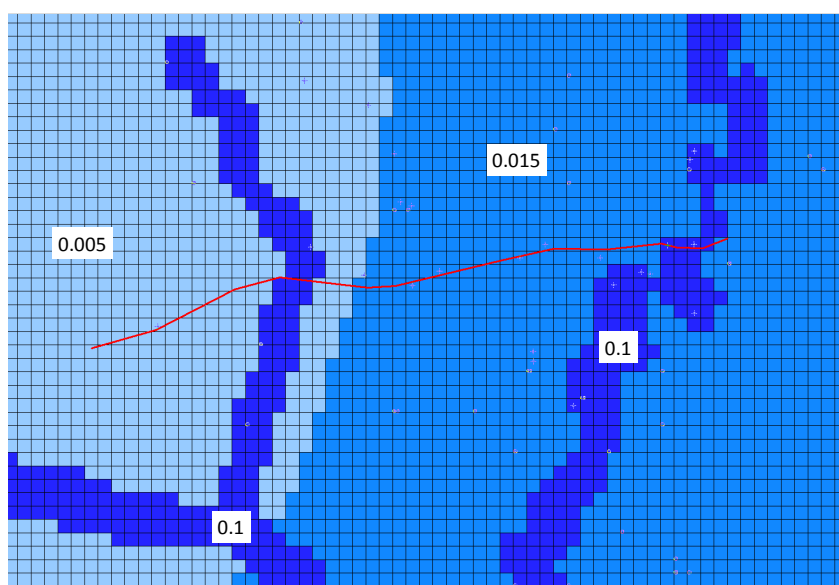
Figure 8 Storage Zones in Wessex Basin Model
