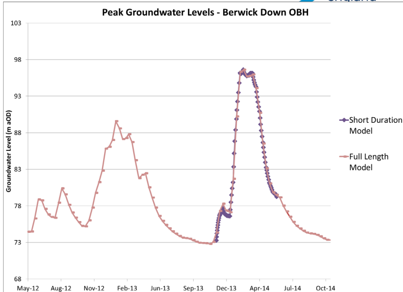
Figure 1 Berwick Down Peak Groundwater Levels
