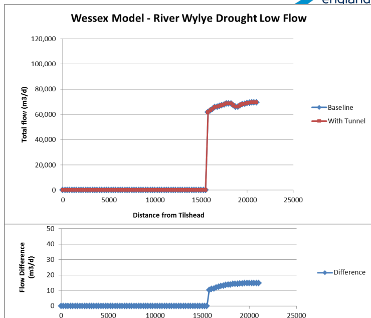
Figure 23 Accretion Plot for Low Flows in River Wylve in the Wessex Basin Model
